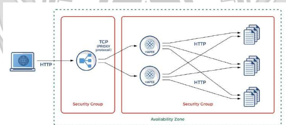
Gambar 2.6 Haproxy
