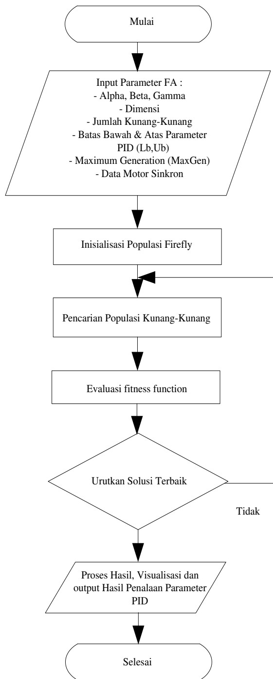
Gambar 3. Flowchart Penelitian
