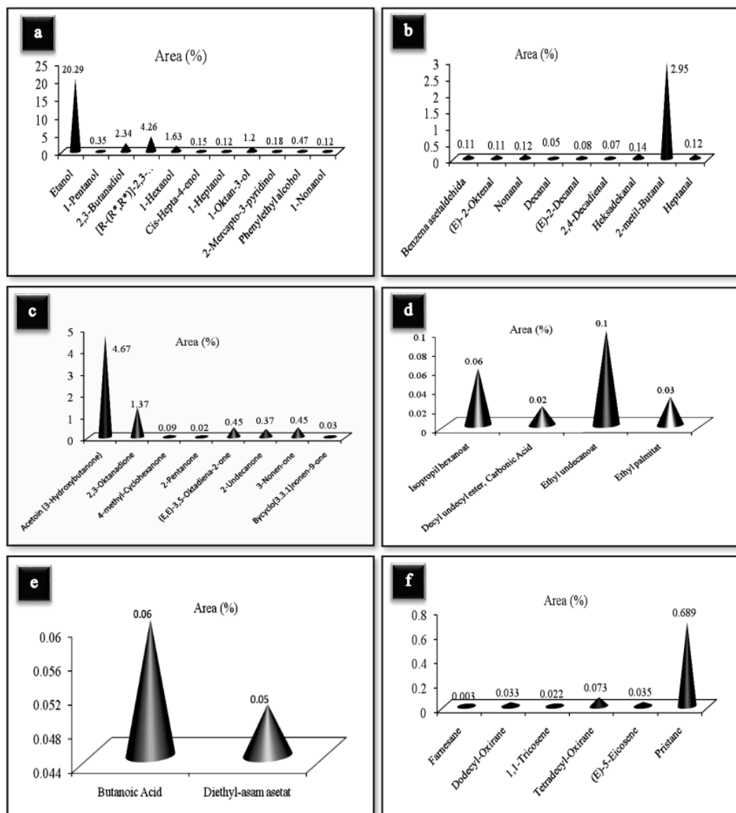
Figure 3. Volatile compounds in Chao teri: a) Alcohols, b) Aldehyde, c) Ketones, d) Ester, e) Organic acid, and f) Miscellaneous compounds
