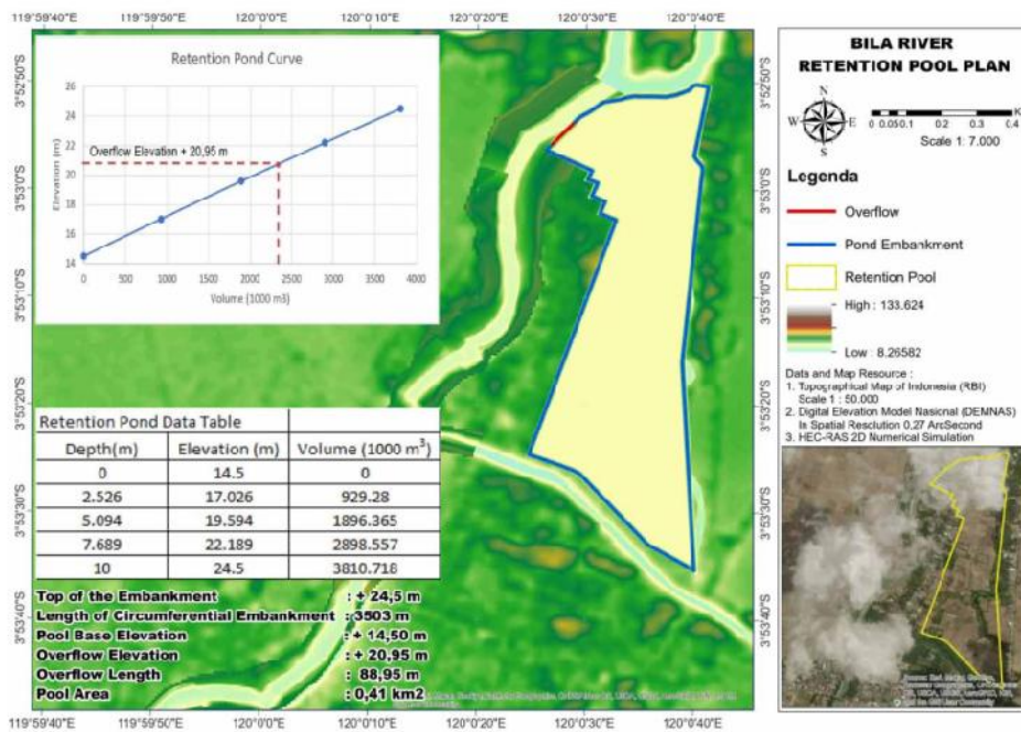
Figure 6 | Bila River retention basin plan.
