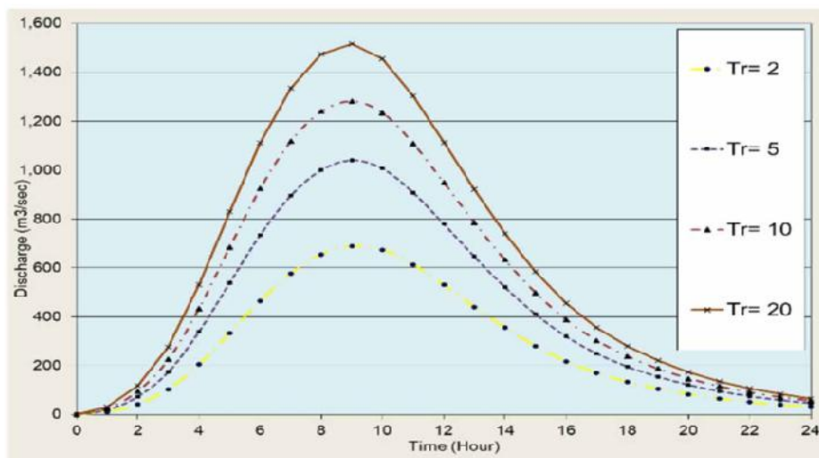
Figure 4 | Superposition SCS synthetic unit hydrograph.
