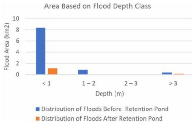
Figure 8 | Graph of area based on flood depth.
