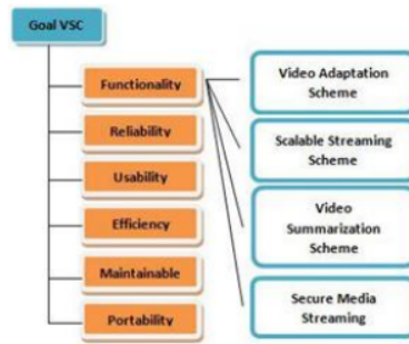
Figure 1. The decision analysis framework
