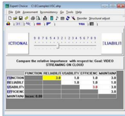
Figure 4. Pairwise comparison of criteria
