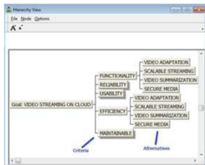
Figure 2. Modeling the decision structure
