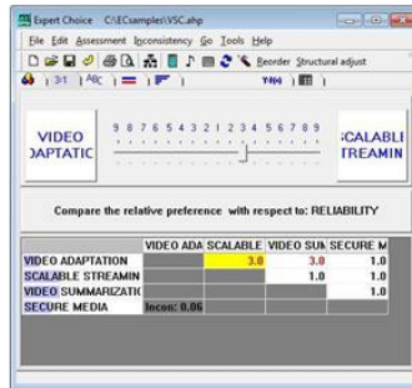
Figure 5. Pairwise comparison of alternative
