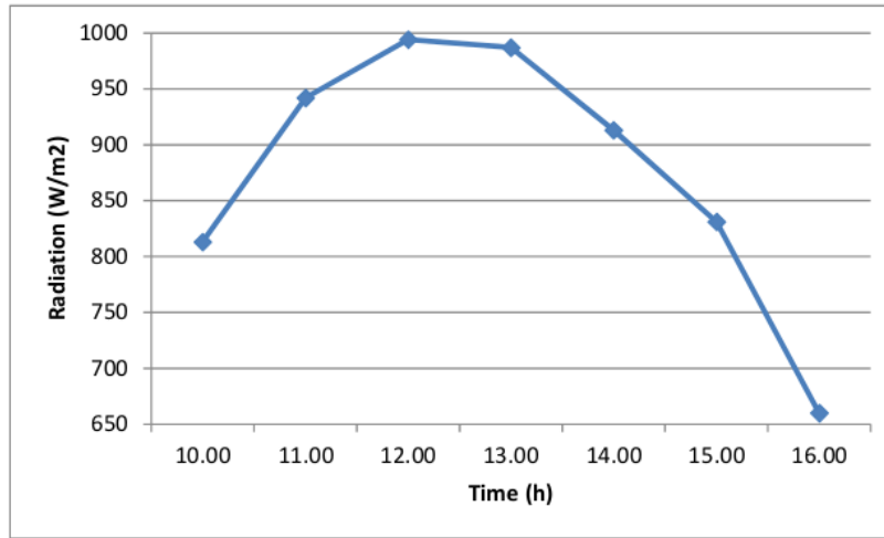
Figure 3: Solar radiation intensity
