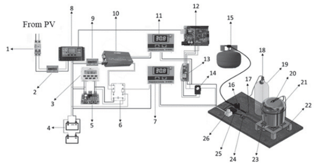
Fig 2. System Circuit Scheme
