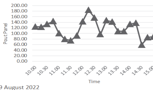
Fig 5. Graph of the panel output power relationship to time
