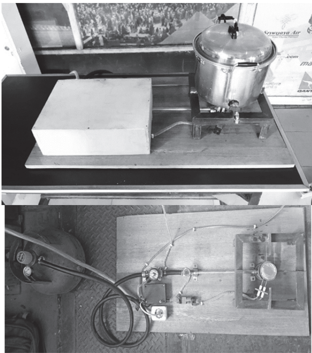
Fig 3. Prototype Kompor Gas Otomatis
