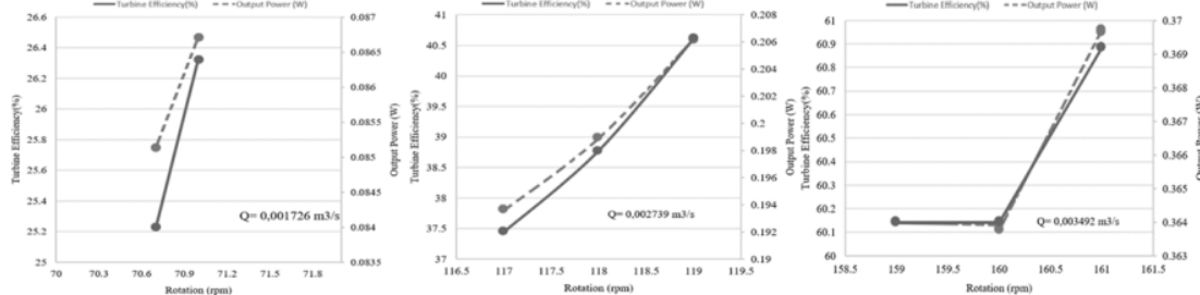
Fig 11. Correlation between speed and turbine efficiency and power output on the four-angle fin test with a slope of 30^\circ
