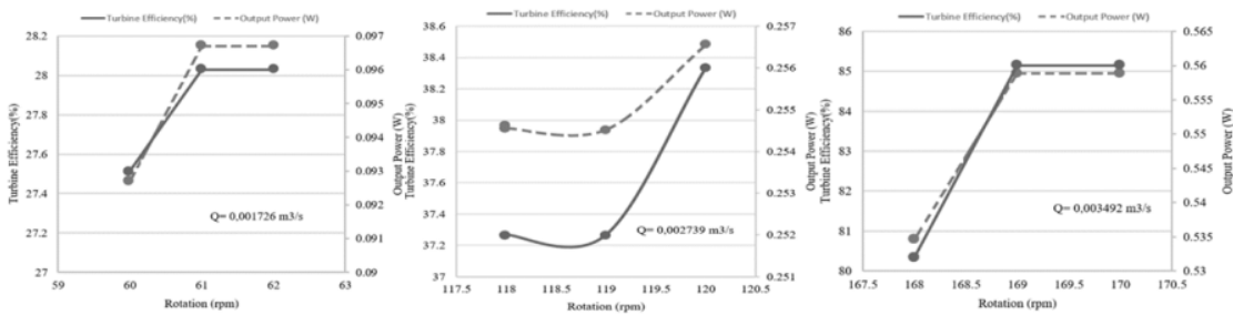
Fig 14. Correlation between rotation to turbine efficiency and output power in the test of two parallel four-angled fins longitudinally tilted at 30°
