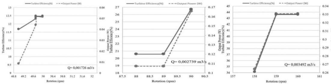
Fig 9. Correlation between rotation and turbine efficiency and output power in the test of two parallel four-angled fins with a slope of 0^\circ
