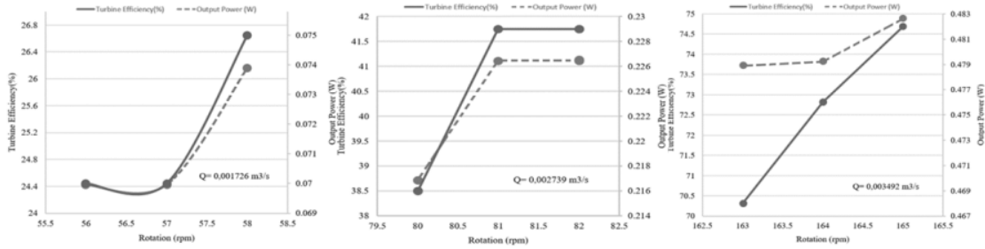
Fig 12. Correlation between rotation and turbine efficiency and output power in the V-shape angled fin test with a slope of 30°
