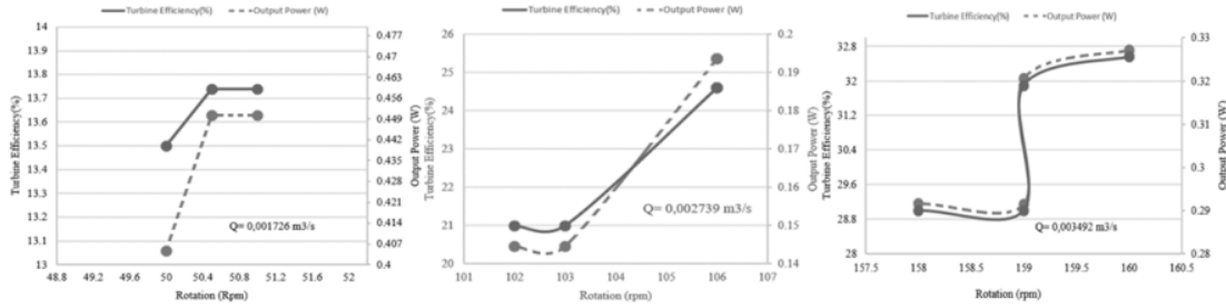
Fig 7. Correlation between rotation and turbine efficiency and output power on the four-angled \Lambda fin test tilted at 0^\circ
