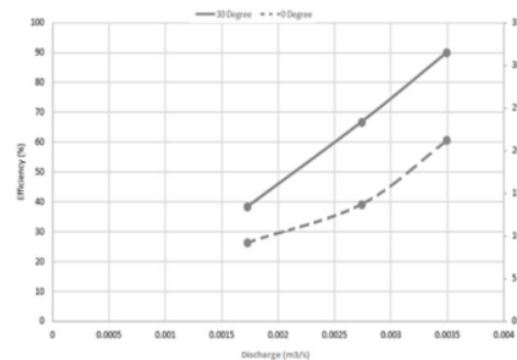
Fig 15. The relationship between testing efficiency (%) to discharge (m 3 /s) with the Elbow-Four Λ type at a slope of 0° and 30°
