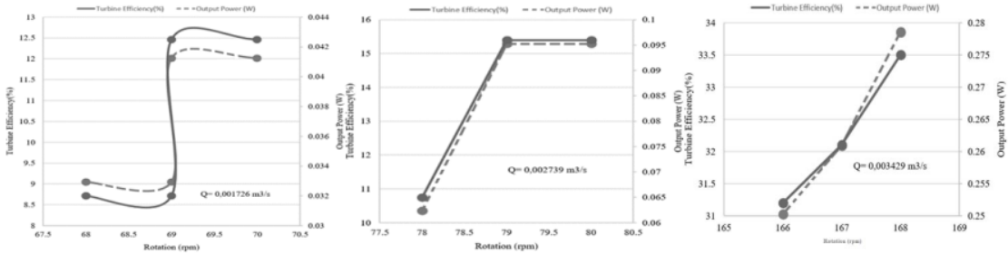
Fig 13. Correlation between rotation to turbine efficiency and output power in the test of two parallel four-angle fins across a slope of 30°
