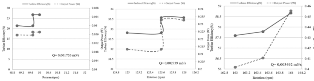
Fig 8. Correlation between rotation and turbine efficiency and output power on the four-angled V-shaped fin test with a slope of 0^\circ
