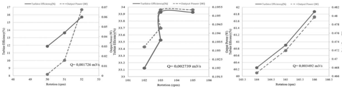
Fig 10. Correlation between rotation and turbine efficiency and output power in the test of two parallel four-angled fins with a slope of 0^\circ
