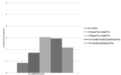
Fig 9. Temperature drop in the test using a water wheel with variations in fin configuration, Q = 0.002739 \text{ m}^3/\text{s} slope of 30^\circ
