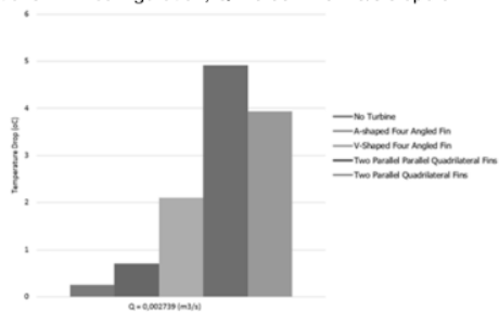
Fig 6. The temperature drop in the test using a water wheel with a variety of fin configurations, Q = 0.002739 \text{ m}^3/\text{s} with a slope of 0^\circ
