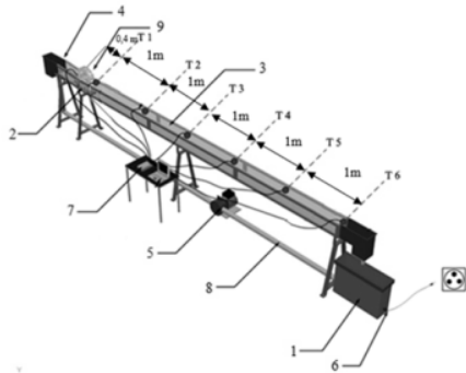
Fig 1. Test scheme
