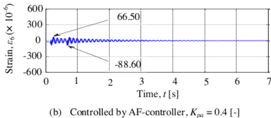
Fig.7. Calculated time history responses of strains at Node 6 for uncontrolled and controlled system due to the base excitation
