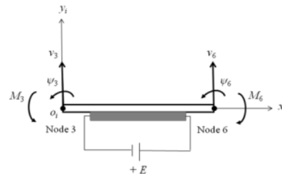
Fig. 5. Modeling of the piezoelectric actuator
