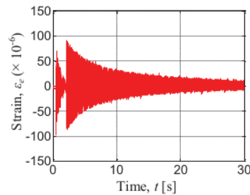
Fig. 11. Experimental time history responses of strains at 0.11 m from the origin of the single-link due to the excitation force generated by the motor's rotation
