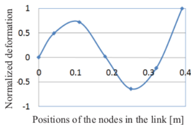
(c) Third vibration mode ( f_3 = 107.19 Hz)
