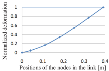
(a) First vibration mode ( f_1 = 6.10 Hz)
