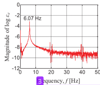
Fig. 8. Experimental natural frequency of the single-link
