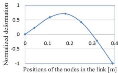
(b) Second vibration mode ( f_2 = 38.22 Hz)
