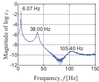
Fig. 9. Calculated natural frequencies of Model I
