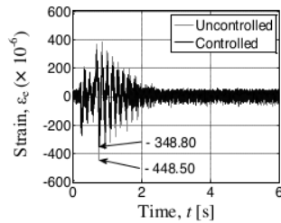
(a) K_p' = 600 applied for both-sides control
