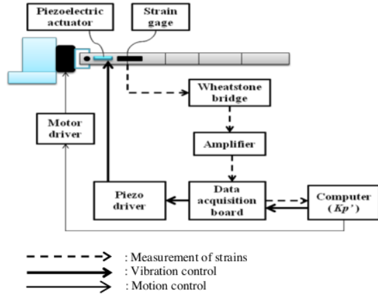
Fig. 17. Schematics of measurement and control system
