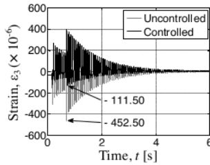
(a) K_p = 600 [Nm] applied for one-side control
