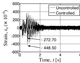
(b) K_p' = 1,000 applied for both-sides control
