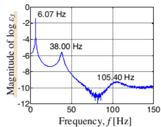
Fig. 10. Calculated natural frequencies of Model I
