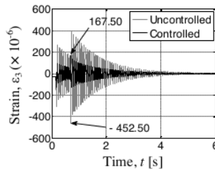
(b) K_p = 600 [Nm] applied for both-sides control
