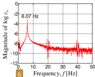
Fig. 9. Experimental natural frequencies of the flexible link
