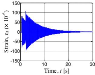
Fig. 15. Calculated time history responses of strains at Node 3 of Model I due to the excitation force generated by the motor's rotation
