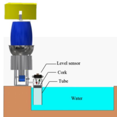
Figure 4. The water level control system.
