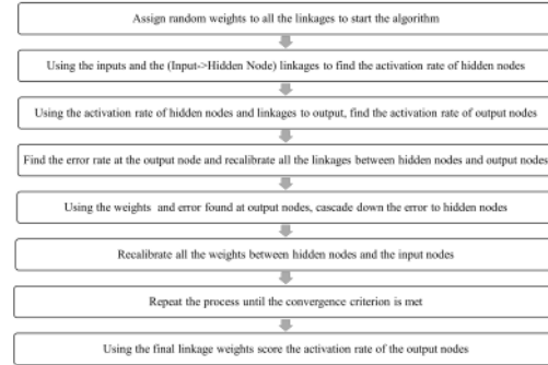
Fig. 1. ANN Algorithm
