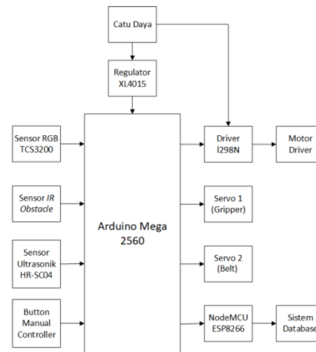
Gambar 1. Blok Diagram Perancangan hardware
