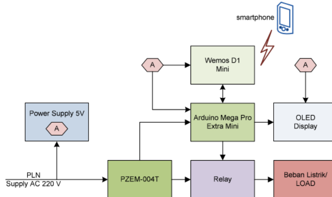
Gambar 7. Blok Diagram Perancangan Hardware
