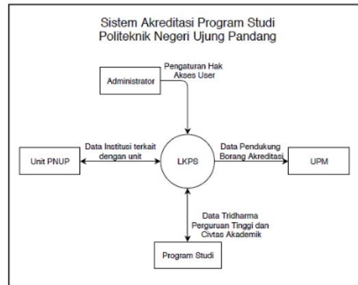
Gambar 7. Diagram Context Sistem Akreditasi PNUP
