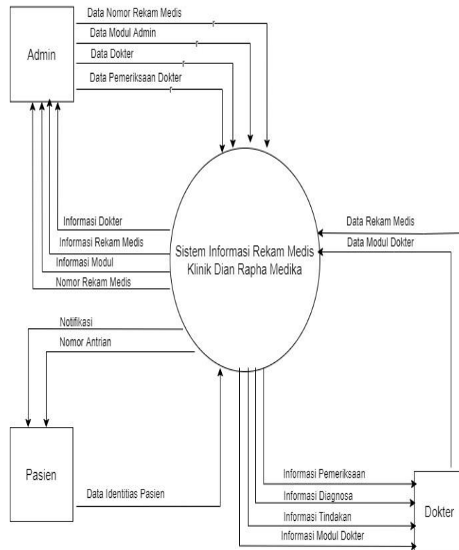
Fig. 3 Context Diagram of Medical Record Information System
