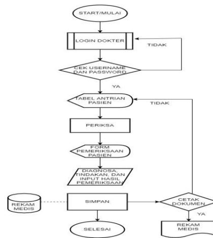
Fig. 2 Flowchart Doctor System
