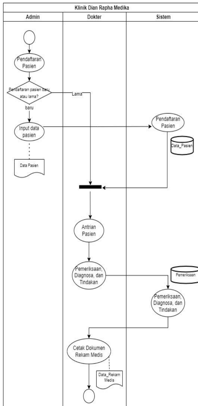
Fig 4. Diagram Activity: Conventional Process and Running System
