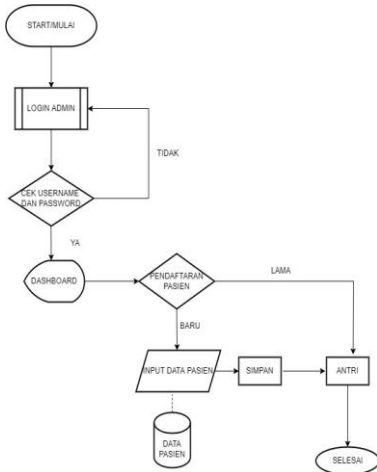
Fig. 1 Flowchart Admin System
