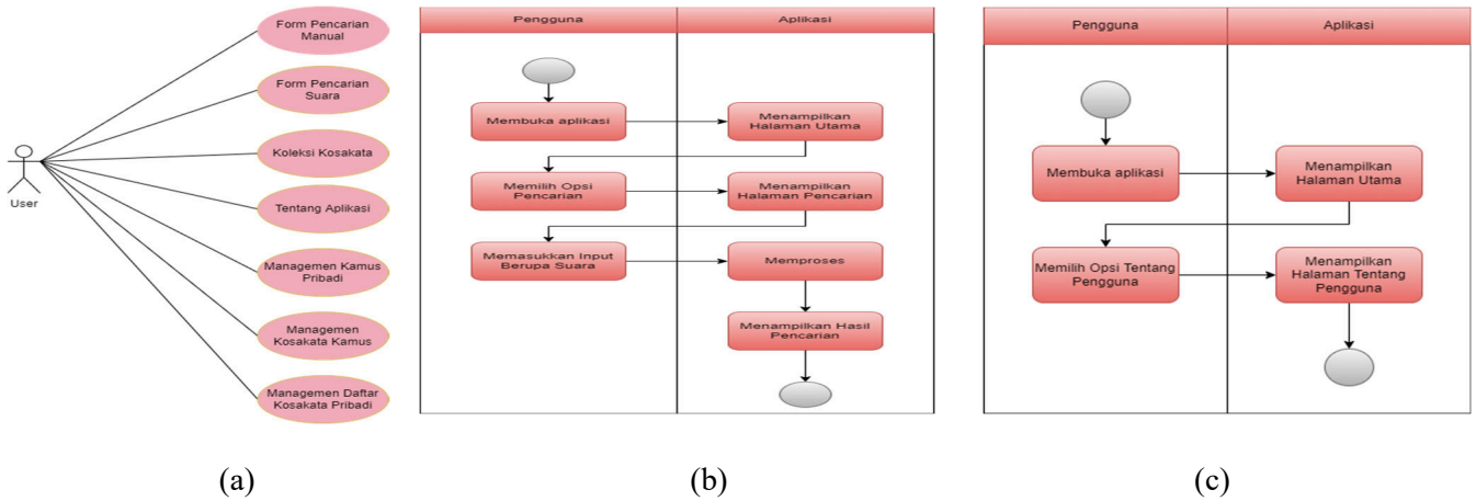
Gambar 3. (a) Use Case Diagram , (b) Activity Diagram Pencarian Suara, (c) Activity Diagram Pengguna
