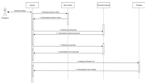
Gambar 4. Sequence Diagram Pencarian Manual
