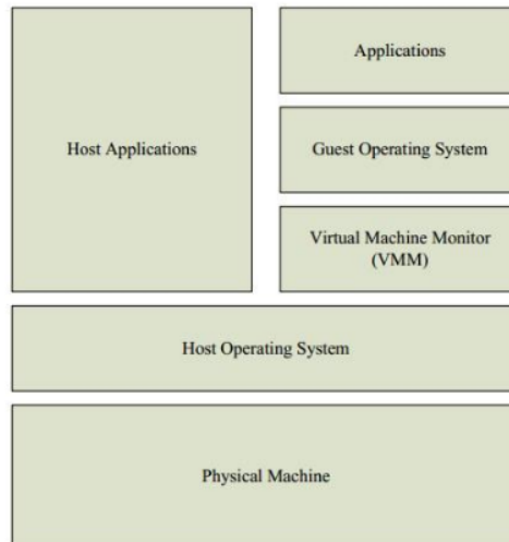
Fig. 1. Virtual machine concept
