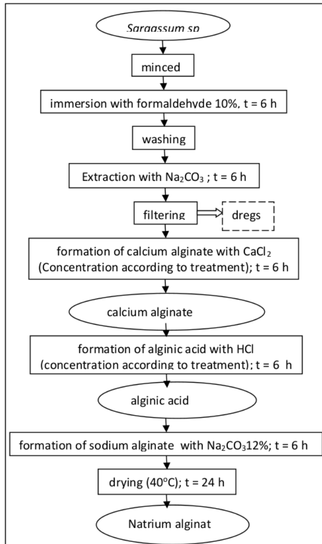
Figure 1. The production process of the sodium alginate extraction process
