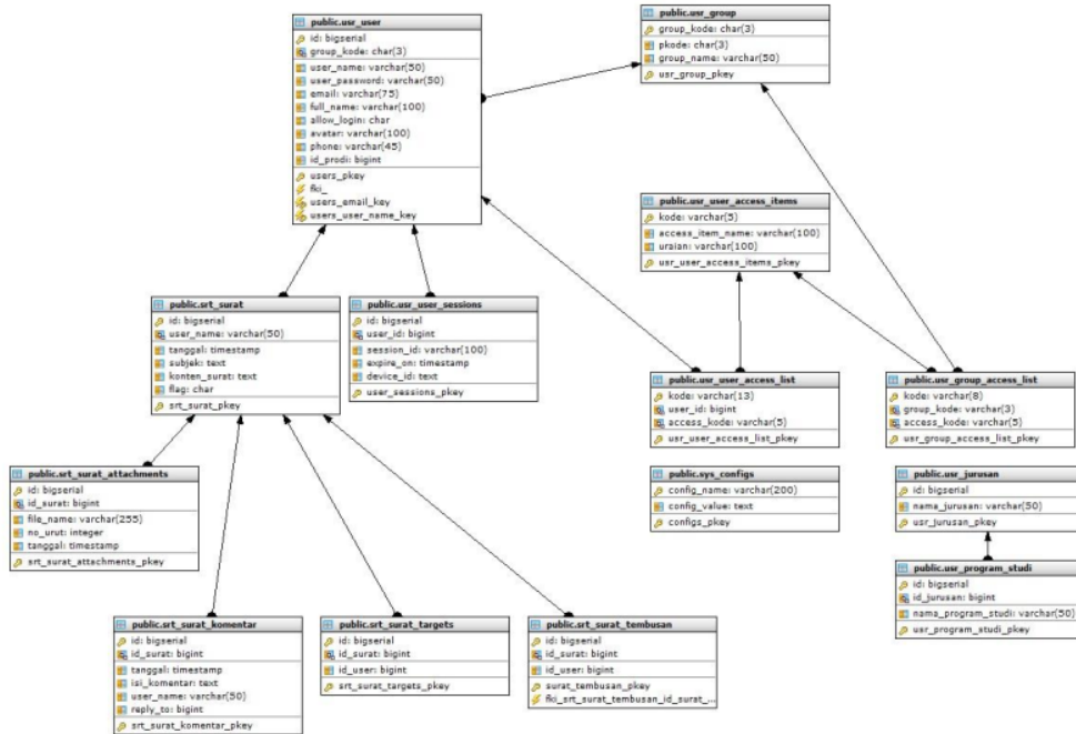
Fig. 4: Database structure
