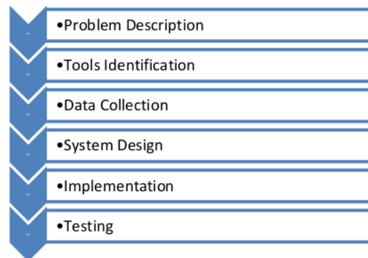
Fig. 1: Research methodology
