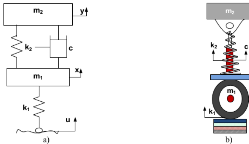
Fig. 1. Mechanism of suspension system on vehicle wheels
