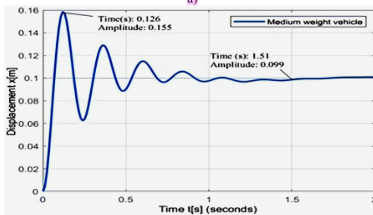
Fig. 8. a) Characteristics of deviation on the vehicle body, b) axle of vehicle with INPUT resistance, U is 0.1 m
