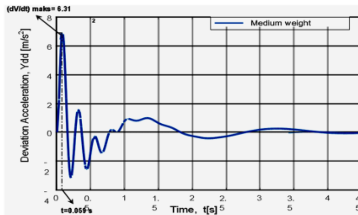
Fig. 10. Deviation acceleration on the vehicle body
