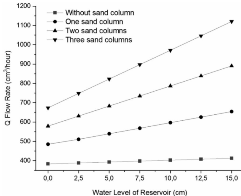
14 Figure 5 | The relationship between the water level above the reservoir and the number of columns to the outflow discharge in the numerical model.
