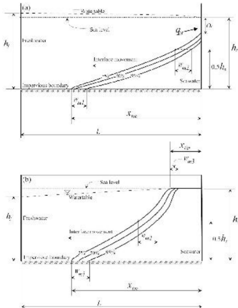
Fig. 1. Conceptual model of an unconfined coastal aquifer subjected to: (a) passive SI and (b) active SI and (modified from Badaruddin et al., 2017).
