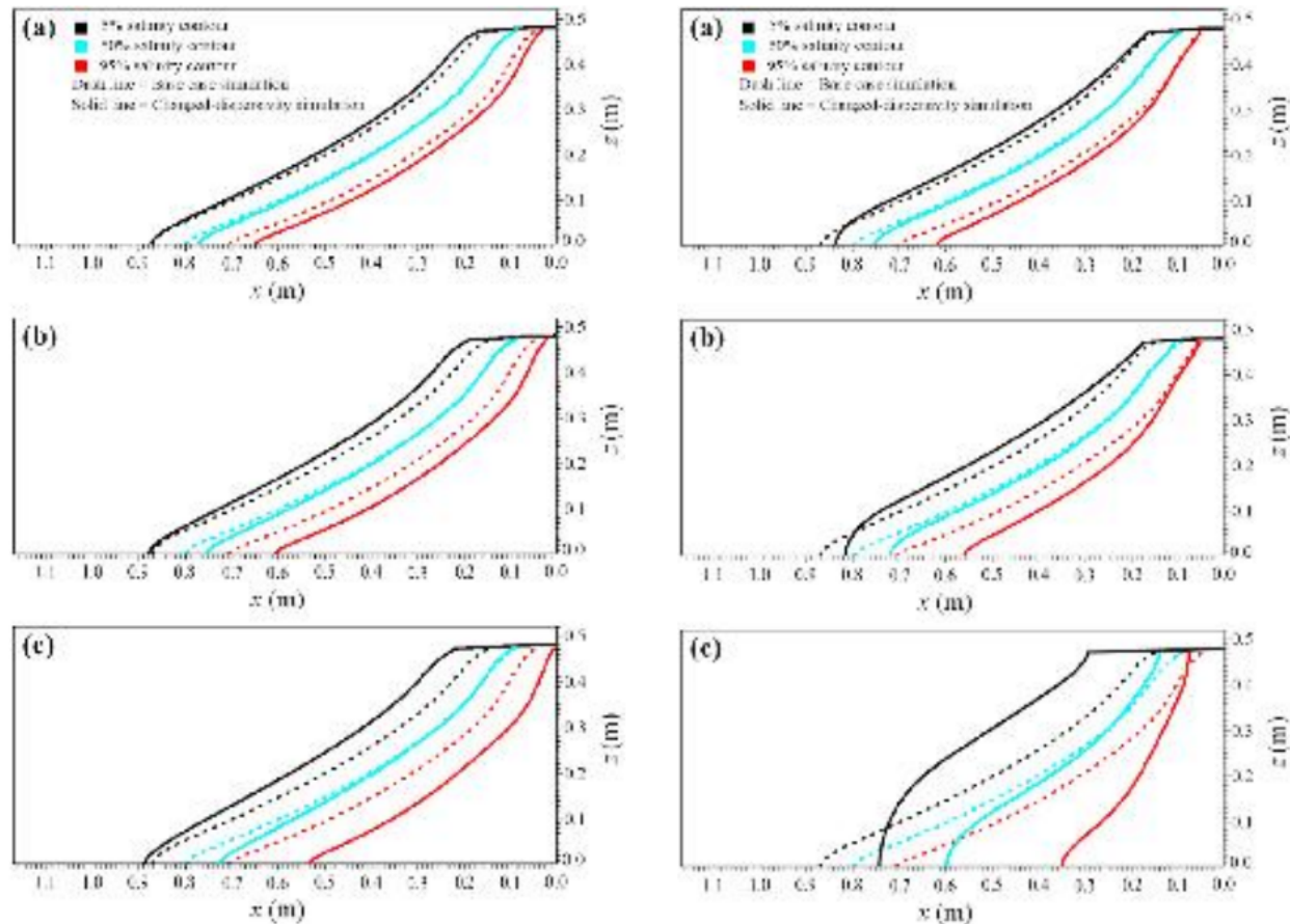
Fig. 14. Comparison of salinity distribution between Case 15 (base case 3) and (a) Case 16 (b) Case 17, and (c) Case 18 at 220 min after steady-state condition (10 min after passive simulation).
