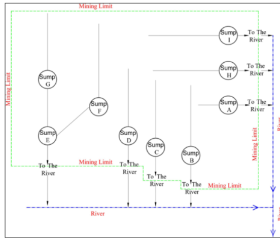
Figure 4. Sump Flow Direction Scheme (Sediment Trap)
