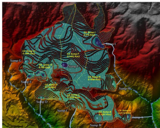
Figure 3. Layout Plan and Catchment Area of Sump.
