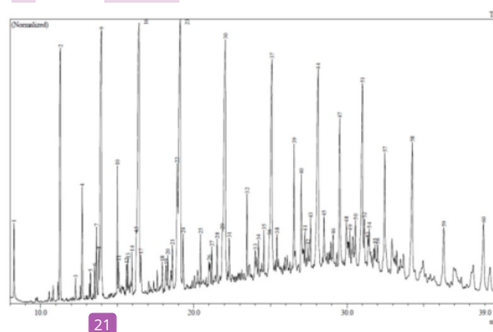
Figure 5. Gas chromatography-mass spectrometry profile for the hexane extract of sea cucumber
