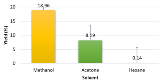
Figure 2. Effect of different solvents to sea cucumber extract yield value.
