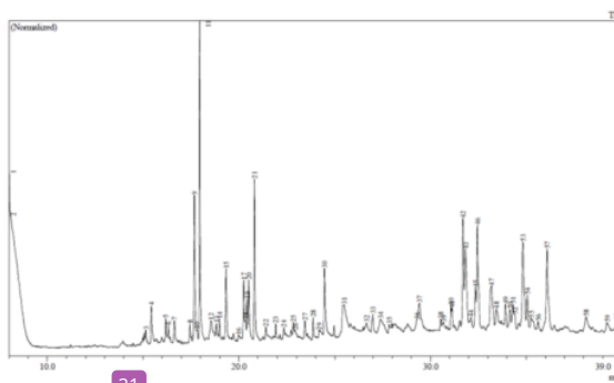
Figure 3. Gas chromatography-mass spectrometry profile for the methanol extract of sea cucumber
