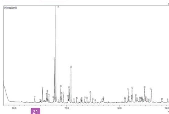
Figure 4. Gas chromatography-mass spectrometry profile for the acetone extract of sea cucumber
