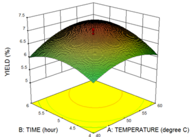
Fig. 1. Response surface plots of yield MSKO.
