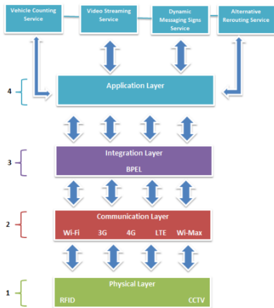
Fig. 1. Conceptual traffic congestion framework for Riyadh City.
