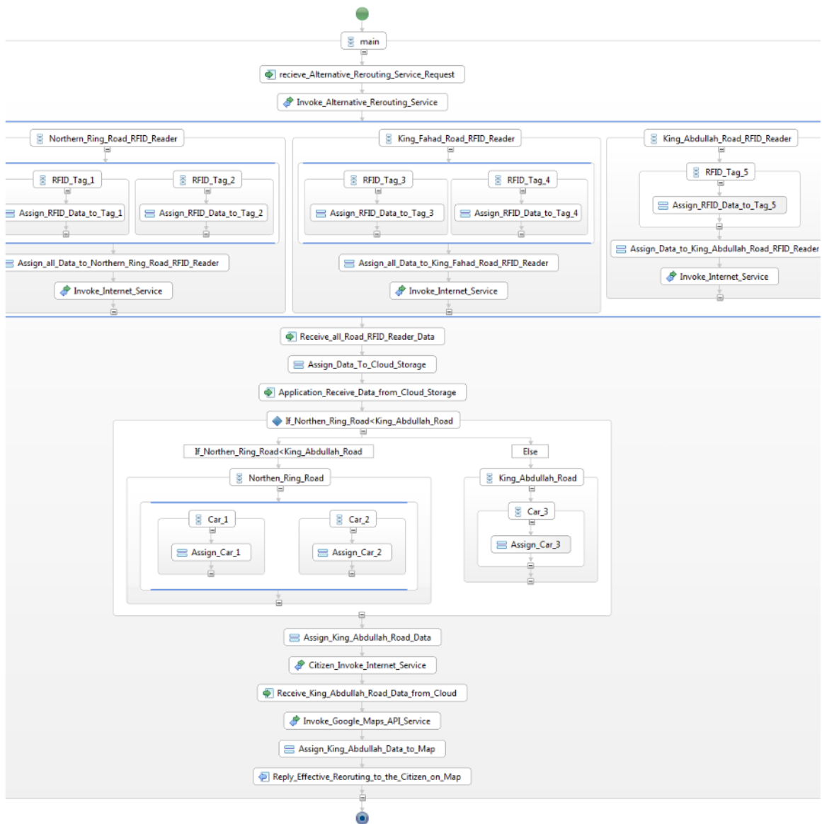
Fig. 13. Alternative rerouting service BPEL Model.
