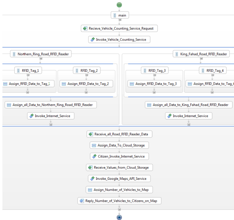
Fig. 6. Vehicle counting service BPEL Model.
