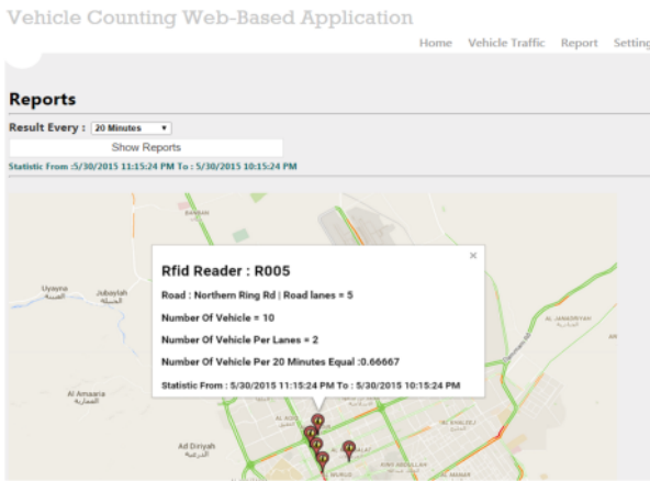
Fig. 7. Vehicle counting service output.
