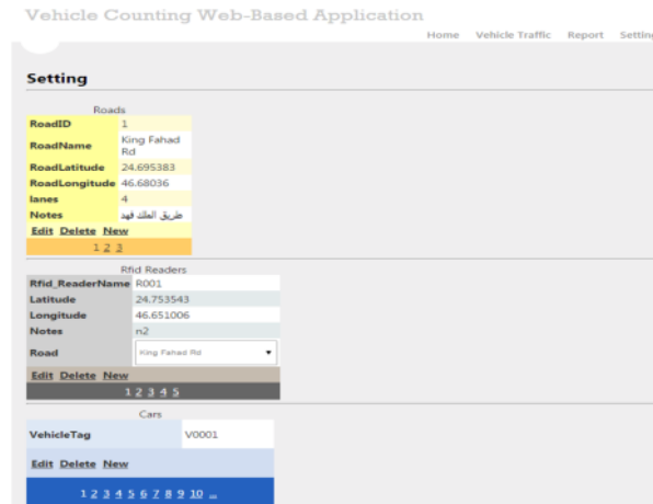
Fig. 4. Setting page in vehicle counting web-based application.
