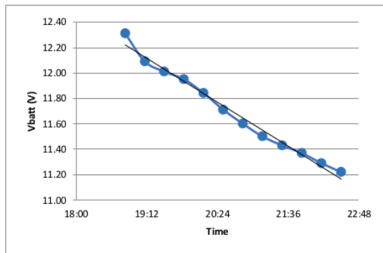
Figure 10. The relationship between battery voltage ( V_{batt} ) and time
