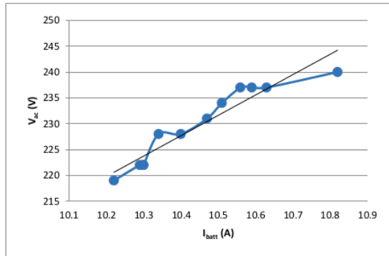
Figure 9. V_{ac} voltage relationship to I_{batt} current
