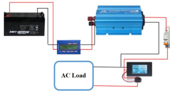
Figure 3. Loaded Battery Testing
