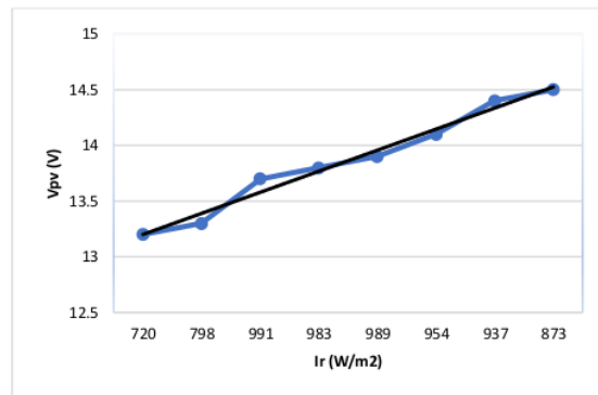
Figure 5. Relationship Between Solar Radiation Intensity and Panel Voltage
