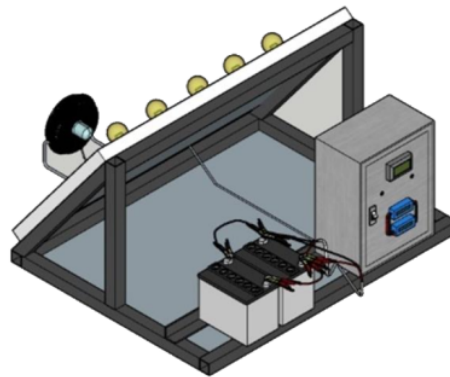
Figure 1. System Prototype
