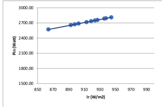
Figure 7. Relationship Between Solar Radiation Intensity and Panel Input Power
