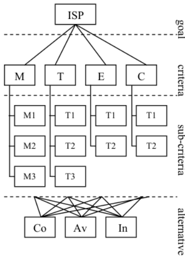
Figure 1. AHP Hierarchy.
