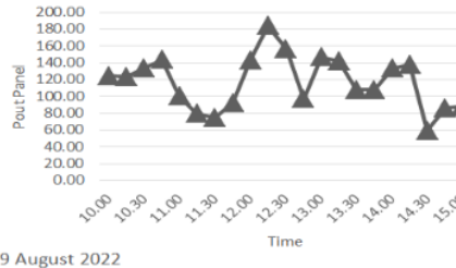
Fig 5. Graph of the panel output power relationship to time
