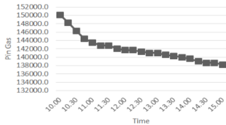
10 August 2022 4 Fig 7. Graph of the relationship between gas input power and time
