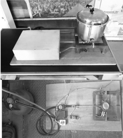
Fig 3. Prototype Kompor Gas Otomatis
