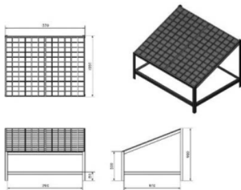
Fig 1. Solar Panel Frame Design
