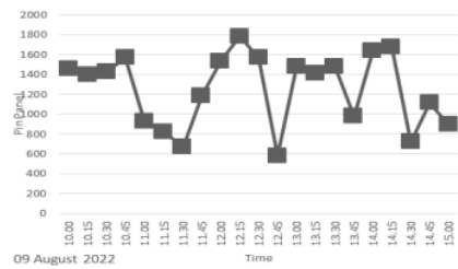
Fig 4. Graph of Panel Input Power relationship to Time
