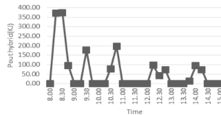
04 August 2022 Fig 12. Graph of hybrid output power against time
