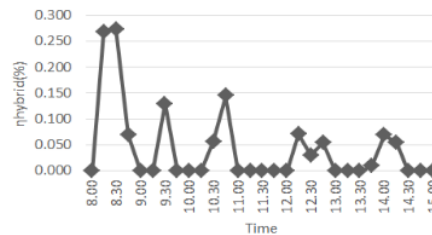
04 August 2022 Fig 13. Hybrid efficiency graph over time
