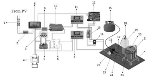
Fig 2. System Circuit Scheme
