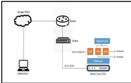
Gambar 2 Topologi Openstack LBaaS
