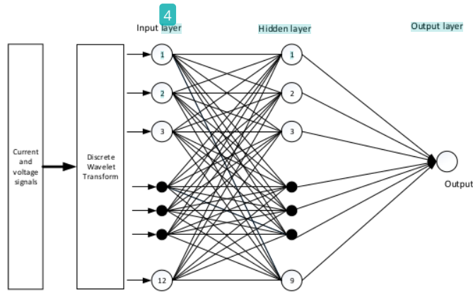
Figure 4. Architecture for WT-ANN of pattern recognition
