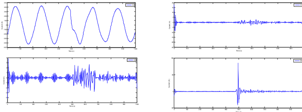
Figure 3. Parts of DWT decomposition for current signals
