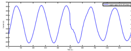
Figure 2. Original signals for SLG-fault current
