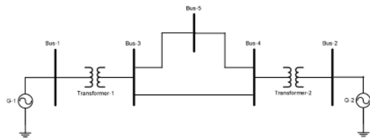
Figure 1. Simulated power system model for ground fault
