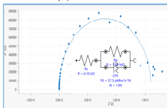
Fig 3: A Nyquist plot for ERGO at 200um Au IDE spacing. The graph represents Z''(\Omega) vs Z'(\Omega) at applied potential 0.2V
