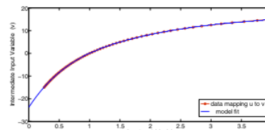
(a) v = f(u)
