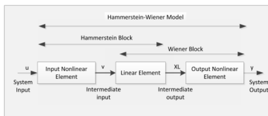
Fig. 1. Hammerstein-Wiener block structure
