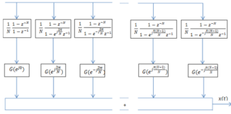
Fig. 4. Diagram of Frequency Sampling Filters
