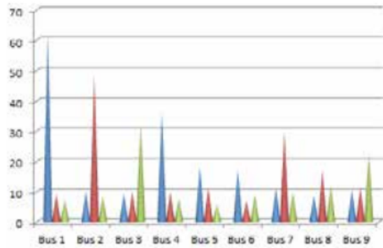
Figure 4. Magnitude of SLGF currents for various fault locations
