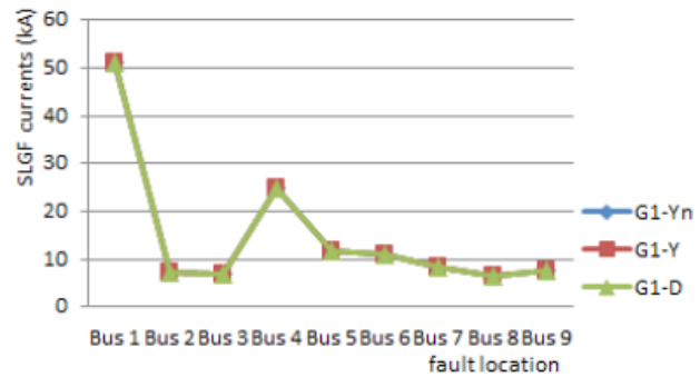
Figure 10. The influence of grounding type of Generator-1 for various buses as fault location at Zn-Zn transformer
