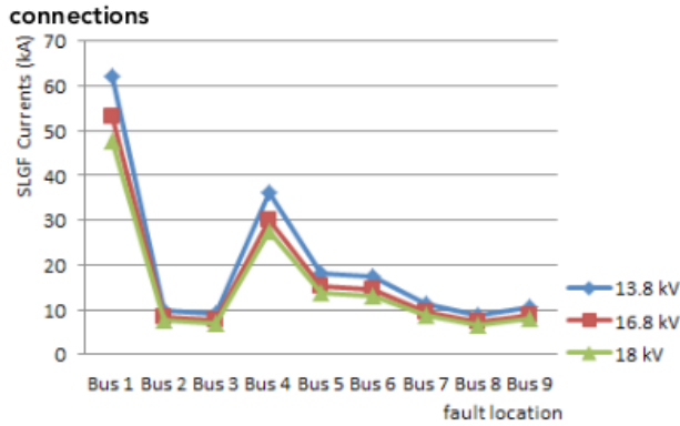
Figure. 11 . The influence of voltage level of Generator-1 for various buses as fault location at Yn-Yn transformer connection
