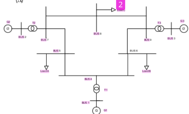
Figure 3. One-line diagram for analysis
