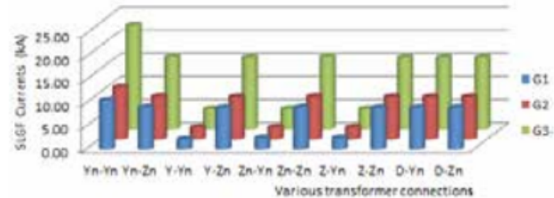
Figure 7. SLGF currents for various transformer connections during ground fault at bus 9
