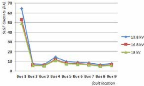
Figure.12 . The influence of voltage level of Generator-1
