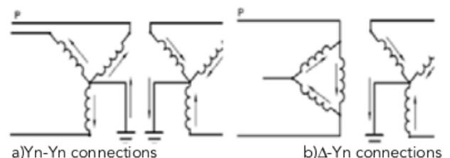
Figure 1. Connection's diagram of Yn-Yn and D-Yn transformer [9]
