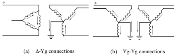
Figure 2. Connection diagram of Δ-Yg and Yg-Yg transformer
