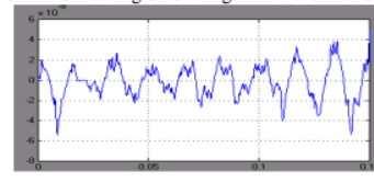
(c) GFC in NGR during SLG at Yg-Δ Transformer Connection
