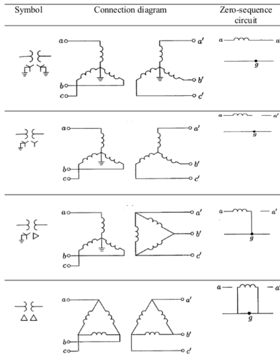
Figure 1. Connection diagram and zero-sequence equivalent circuits [5], [11]
