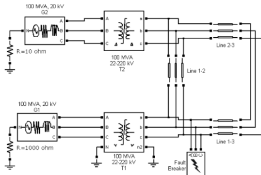
Figure 3. One line diagram for simulation
