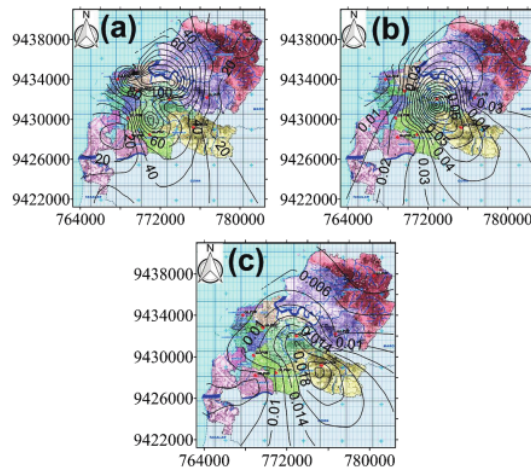
Figure 5. Map of (a) the depth of groundwater aquifer in Makassar City (units in m), (b) the optimum groundwater pumping discharge in Makassar City (units in m^3/min ), and (c) the groundwater aquifer transmissivity in Makassar City (units in m^2/min )
