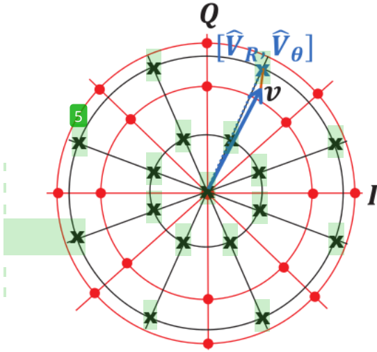
Fig. 5. Phase plane for joint quantisation.
