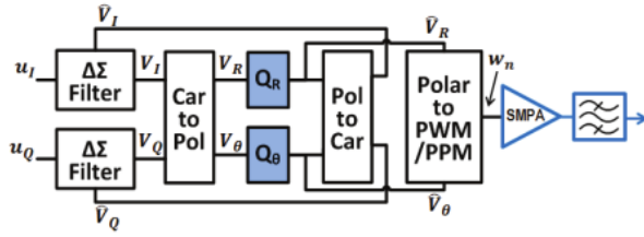
Fig. 2. Cartesian \Delta\Sigma with polar quantisation.
