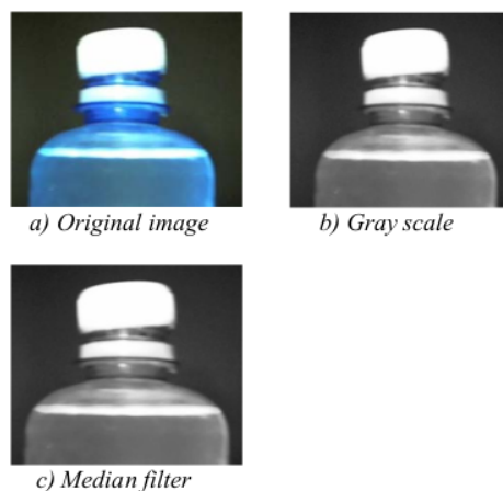
Figure 3. The result of gray scale and median filter for a misplaced cap
