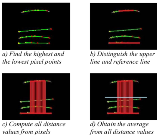
Figure 5. Feature extraction method for a misplaced cap
