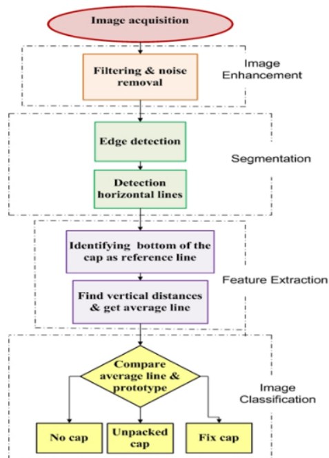
Figure 2. Proposed AVI for cap inspection
