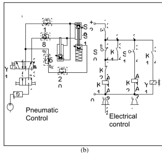
Figure-3. (a) Simulation of wheel suspension loading with pneumatic actuators (b) Control of electro-pneumatic system.
