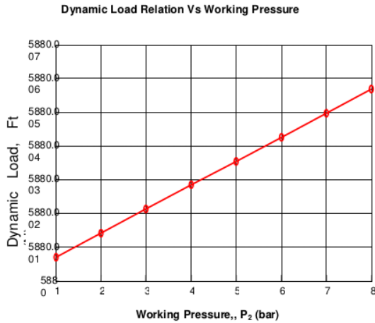
Figure-4. Dynamic load characteristics of pneumatic systems.
