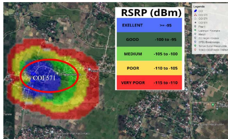
Figure 4. RSRP Coverage Simulation Results.
