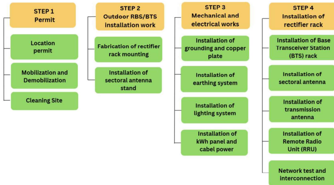
Figure 6. Block Diagram of Combat-571 Installation.
