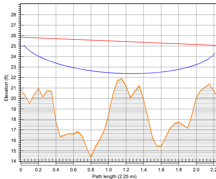
Figure 5. Microwave Link Simulation Results.
