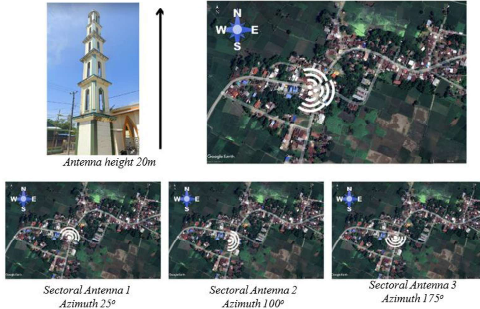
Figure 3. Antenna Placement and Orientation Design.
